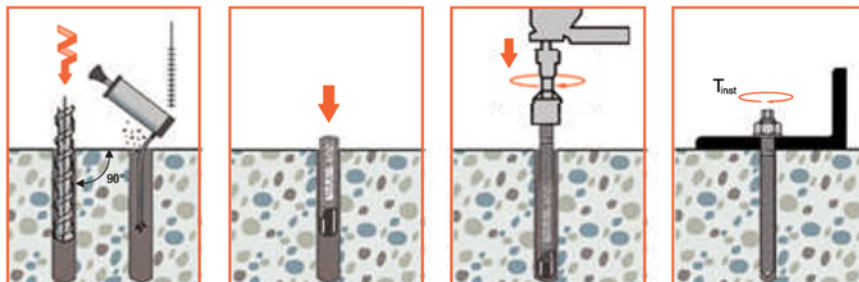
Drill hole and thoroughly clean (brushing and blowing)
